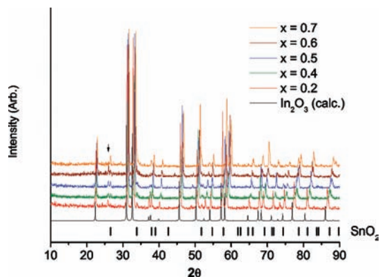
Figure 3. XRD patterns of high-pressure products for x = 0.2 – 0.7 and the calculated XRD pattern of corundum \text{In}_2\text{O}_3 (no \text{K}_{02} ). The peak positions for \text{SnO}_2 (PDF #41–1445) are marked below the XRD patterns. The peak at 2\theta \sim 25^\circ corresponding to the unknown phase is indicated with an arrow.
